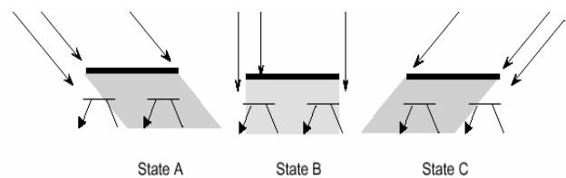
Fig. 1 Alternative solar tracking method
